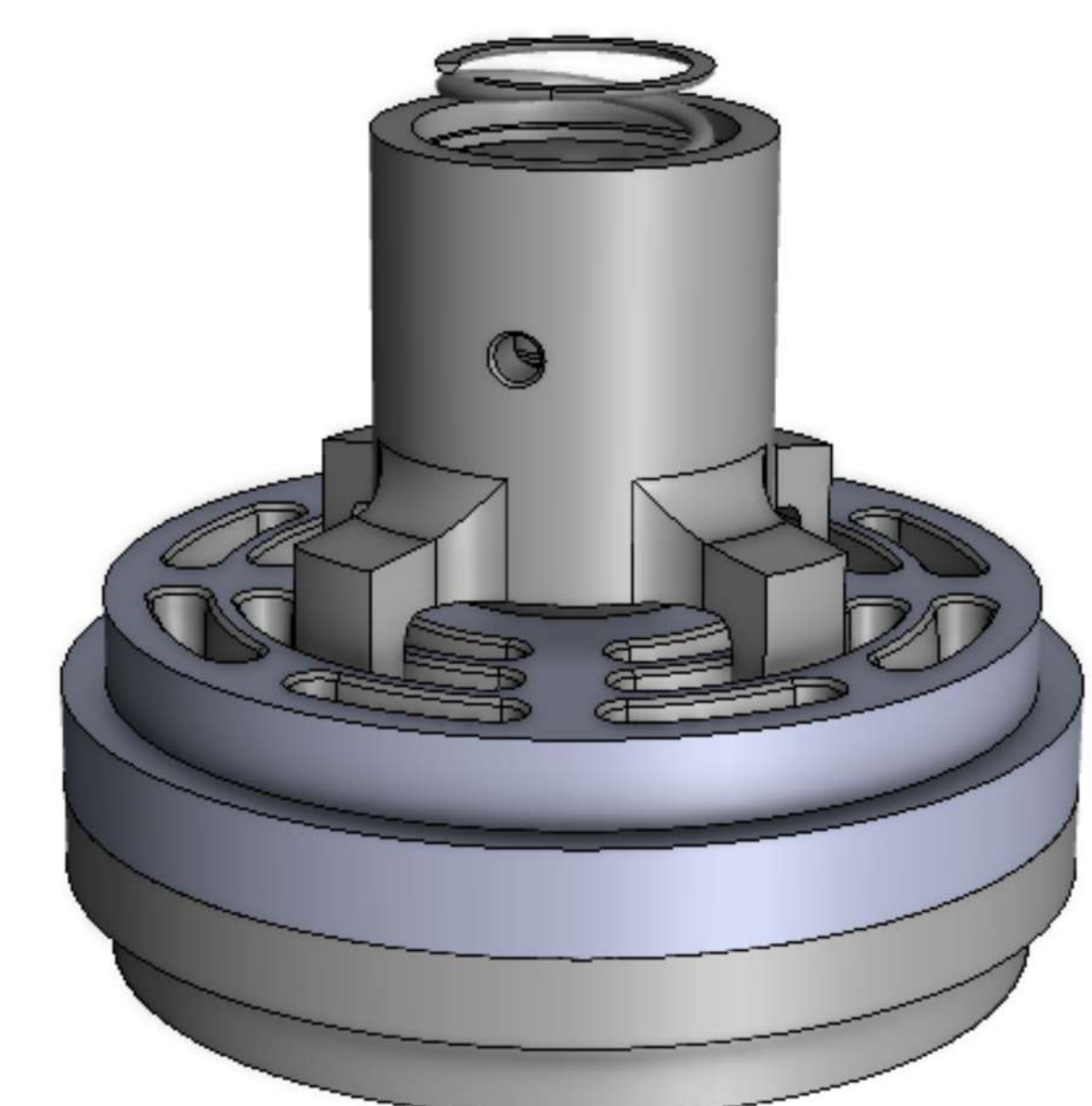
3rd Stage Suction Valve
