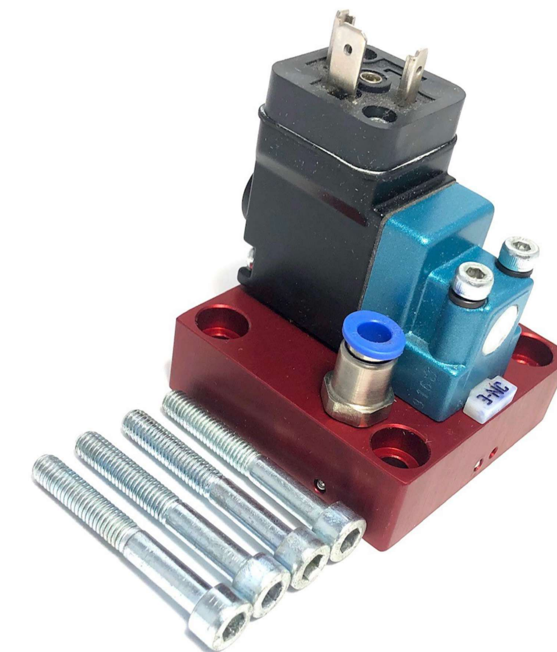
Cover plate exhaust UMS-CPE-COMPACT
