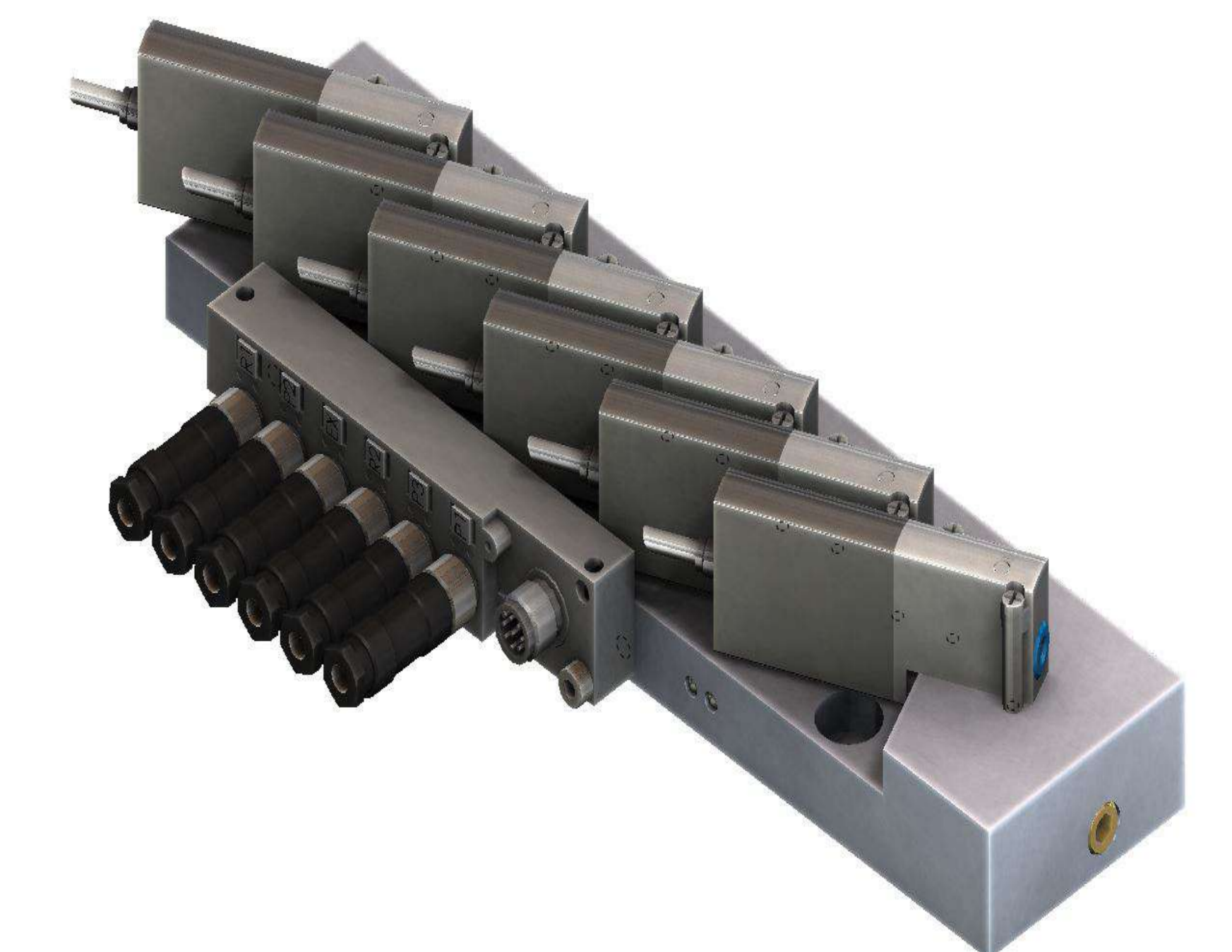
Cover with valve 0002-604-90-30
