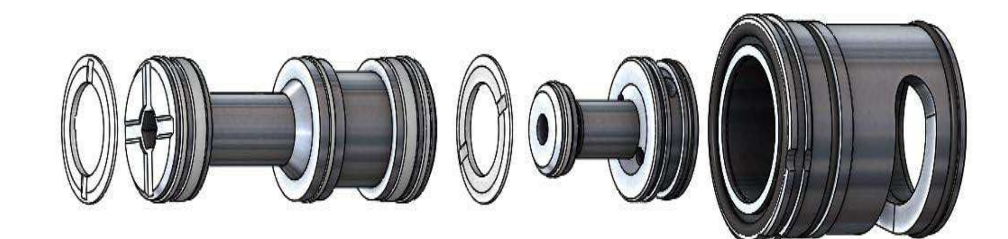
Exhaust rebuilt piston parts 0002-602-90-46
