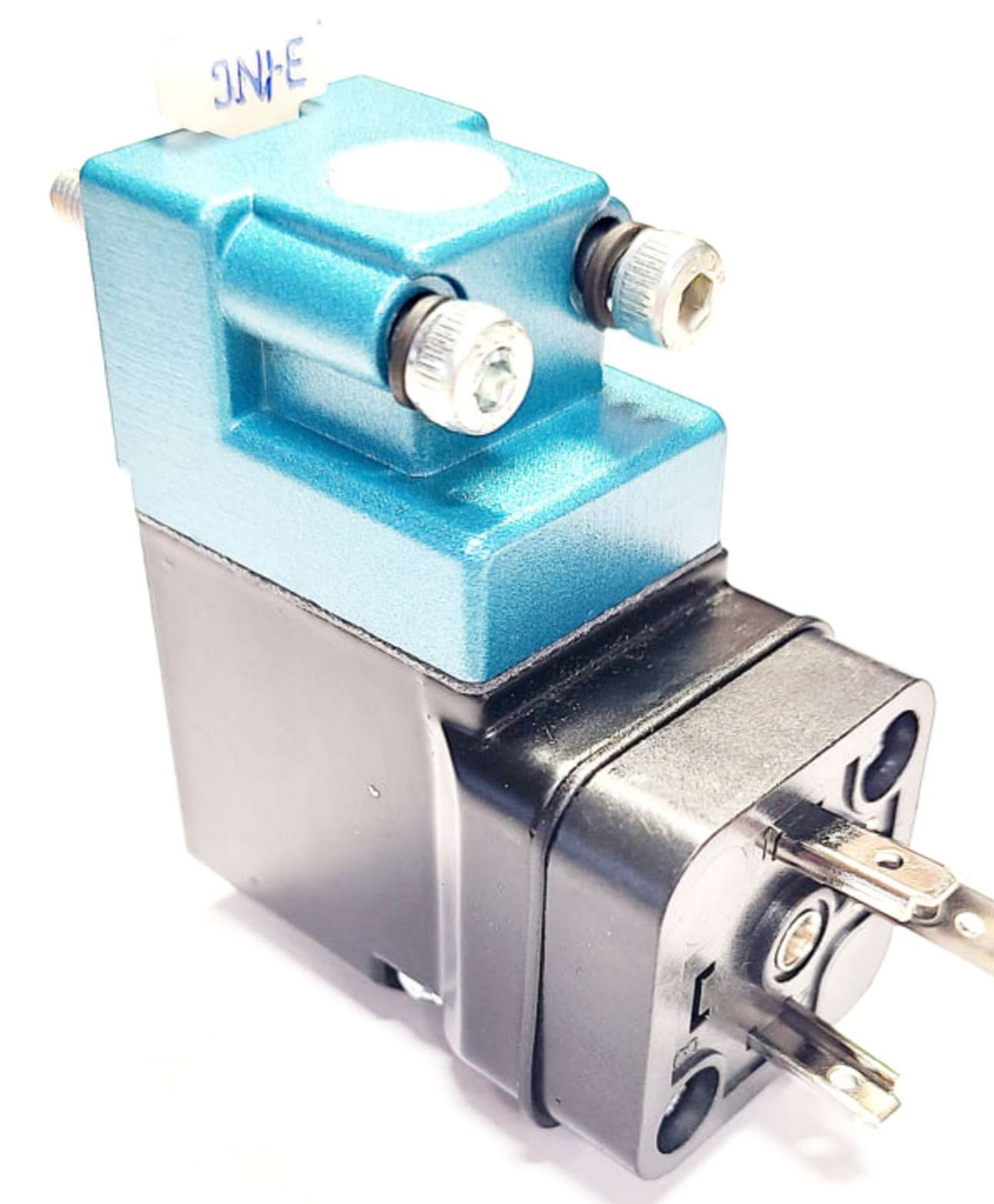
Pilot valve VPU24VDCNO/NC:8590
