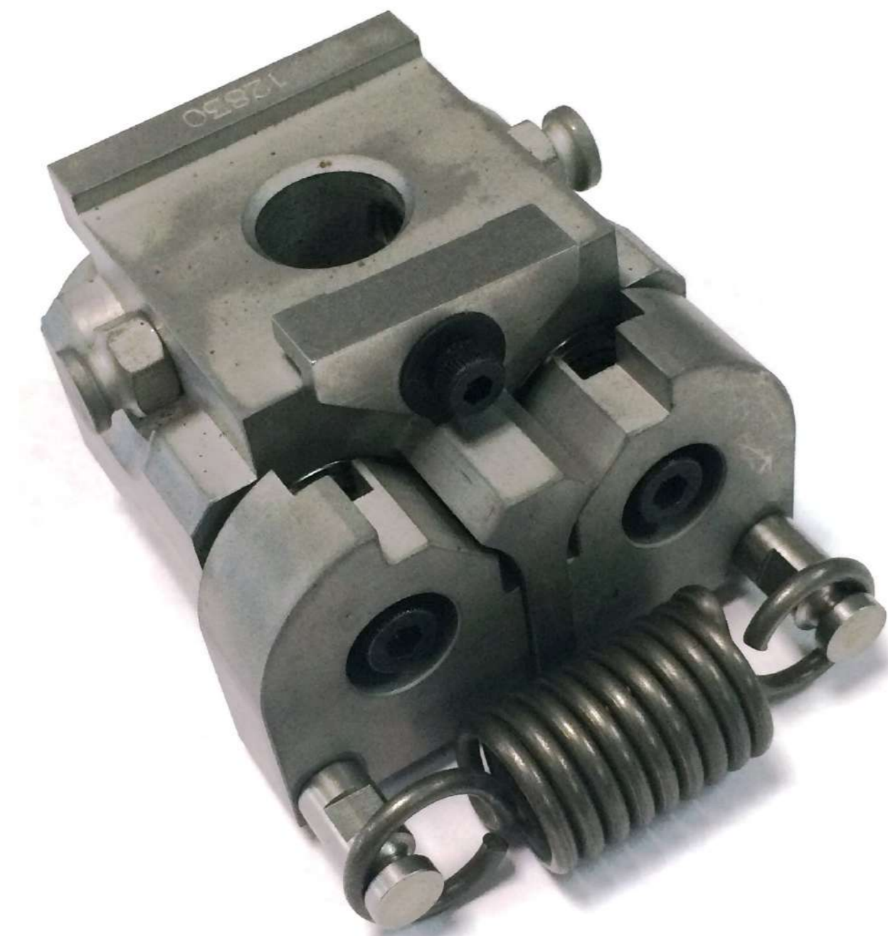
S2 Gripper holder ass'y
