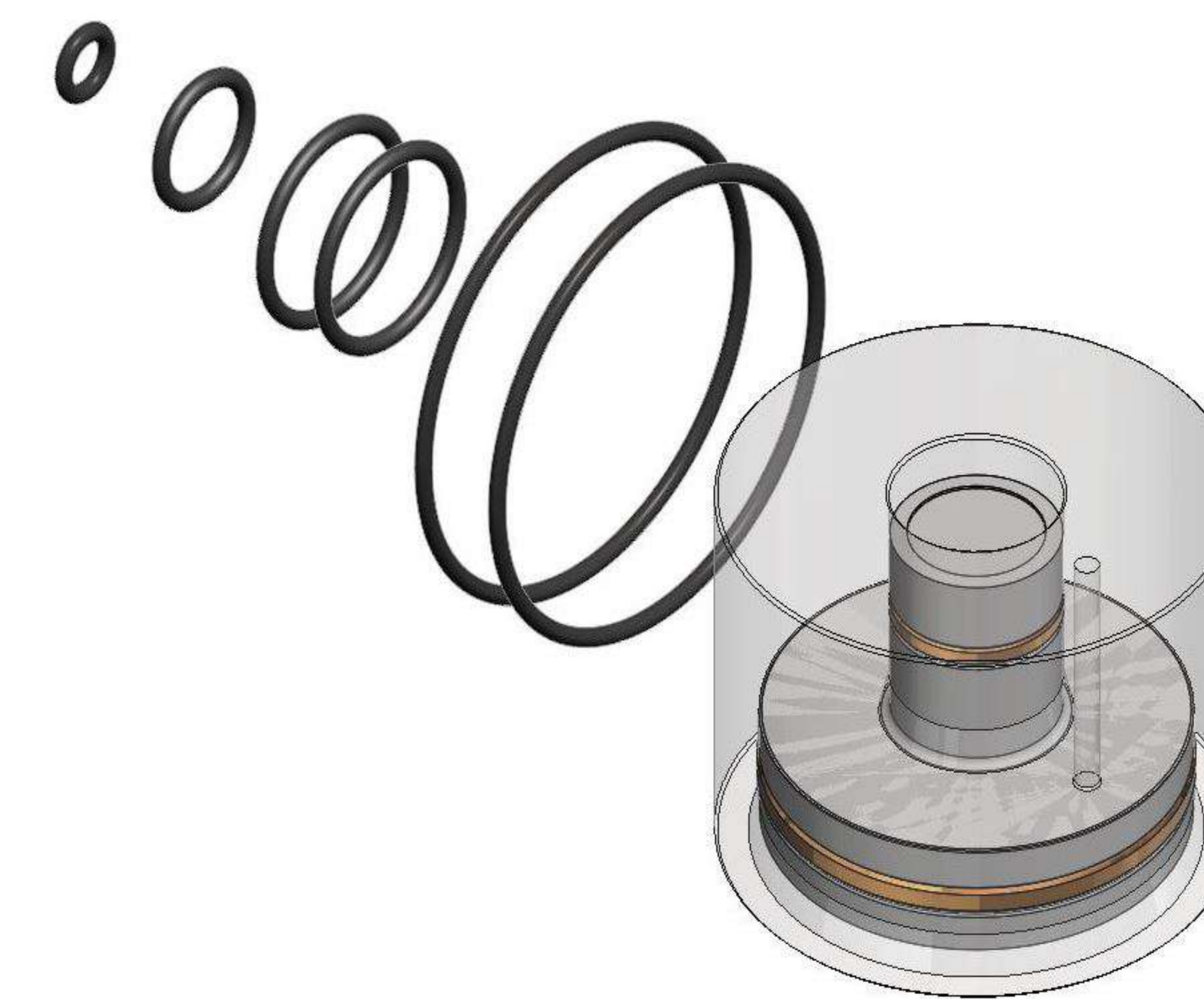
ECO valve maintenance parts UMS-114583-ECO-KR
